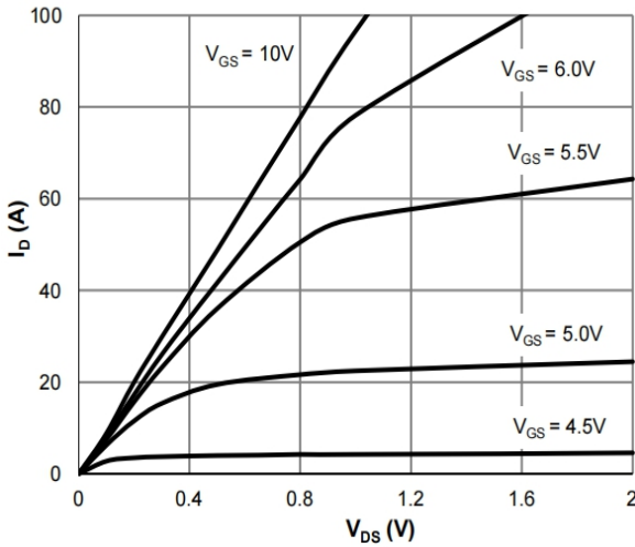
Figure 1: Saturation Characteristics
